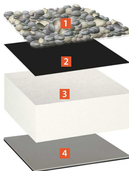
Inverted roof indicative build-up
