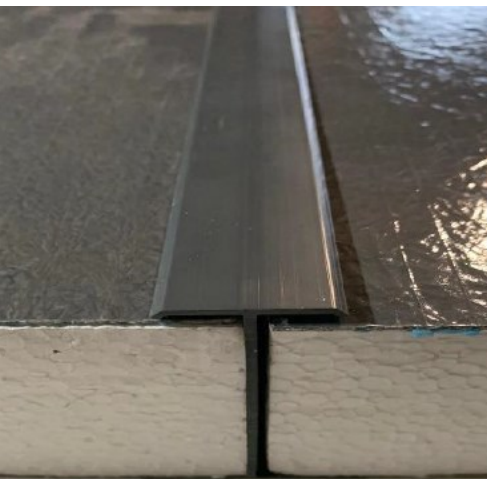
Bauder JFRI Upstand Board
