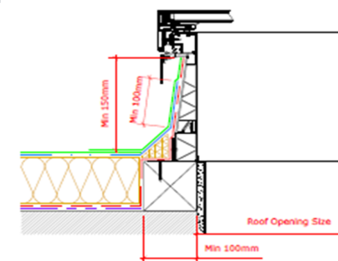
Fixed ventilated with vertical tapered upstand
